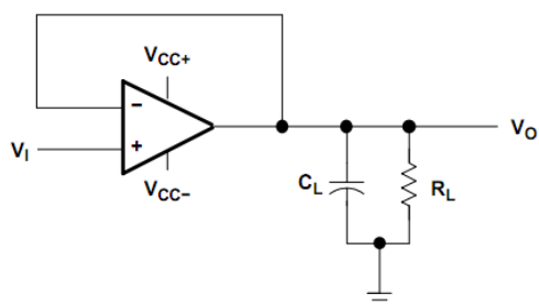
Figure11: Unity-Gain Amplifier
