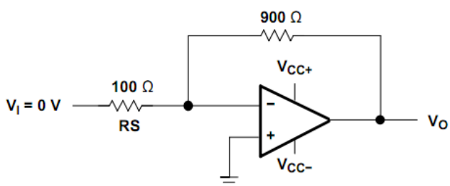
Figure 12: Noise-Test Circuit
